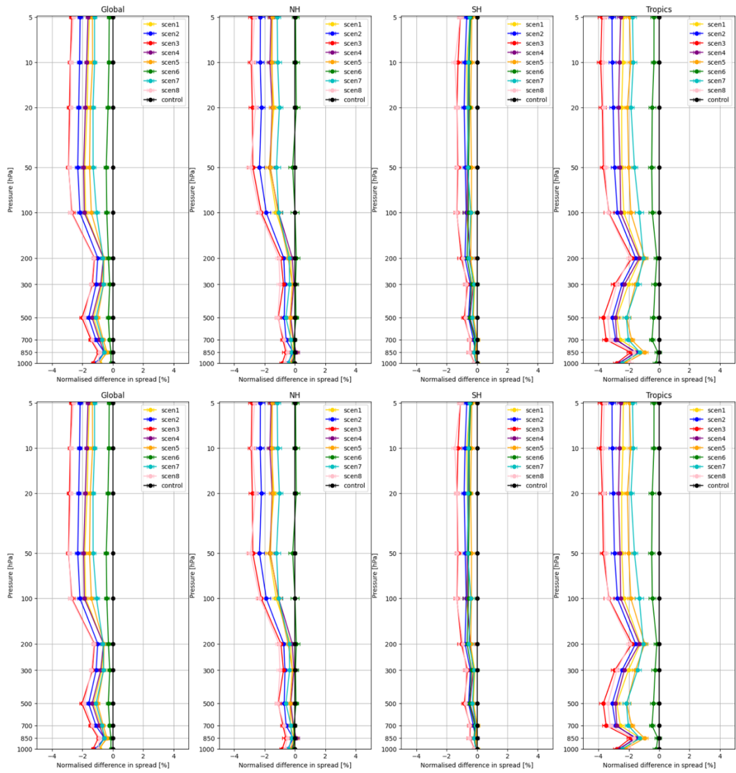
Figure 6 The percentage temperature (upper panel) and zonal wind (lower panel) spread reductions for 12-hour forecasts, relative to the control experiment given on fixed
