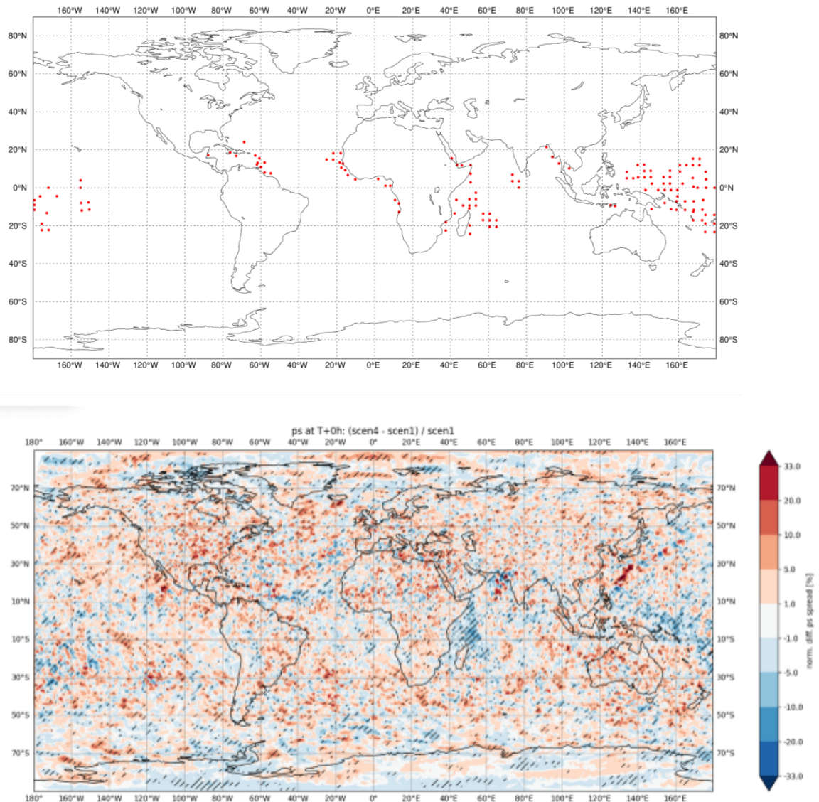
Figure 8 Upper panel: locations of marine observations used in SC 4. Lower panel: The analysis surface pressure uncertainty reductions comparing SC 4 with SC 1, for June 1-30, 2023. Blue shading indicates that the marine observations in SC 4 are reducing the surface pressure analysis uncertainty when compared with SC 1.
