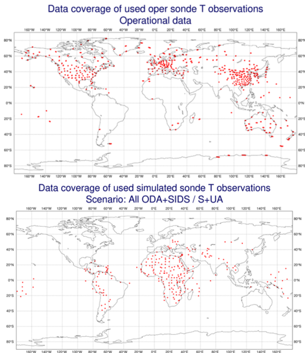
Figure 2 Spatial coverage of radiosondes measurements used in a 12-hour assimilation window on June 1, 2023. Real radiosonde observations are shown in the upper panel and the simulated observations used in SC 3 (All ODA+SIDS / S+UA) are given in the lower panel. Note, the slight horizontal drift in the location of real radiosondes, but not seen with the simulated data. The simulated radiosondes are assumed to have a fixed location in this study.
