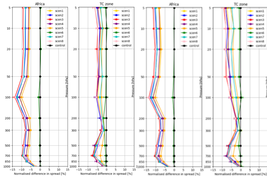
Figure 9 Zonal wind spread reductions for 12-hour forecasts for the Africa region (left) and main development region (“TC zone”) (right). Similar spread reductions are found for temperature, humidity and meridional wind.
