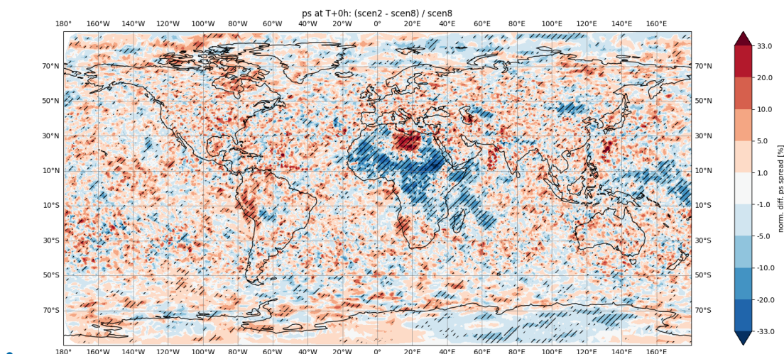
Figure 11 The percentage difference in surface pressure analysis uncertainty comparing scenario 2 with SC 8. Blue shading indicates that SC 2 has a smaller surface pressure uncertainty than SC 8.
