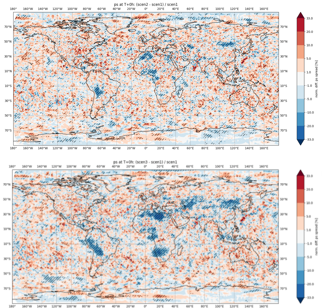
Figure 10 The additional surface pressure analysis uncertainty improvements when SC 2 is compared with SC 1 (upper) and when SC 3 is compared with SC 1(lower).
