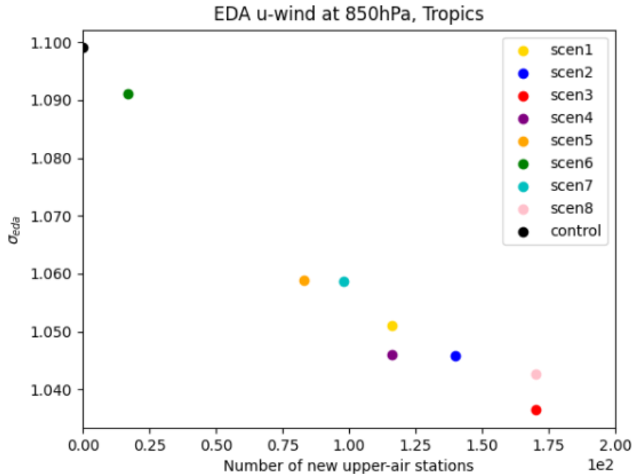
Figure 7 The change in short-range forecast uncertainty for the zonal wind ( \text{m s}^{-1} ) at 850 hPa in the tropics, plotted as a function of the number of new upper-air observation sites in the tropics.
