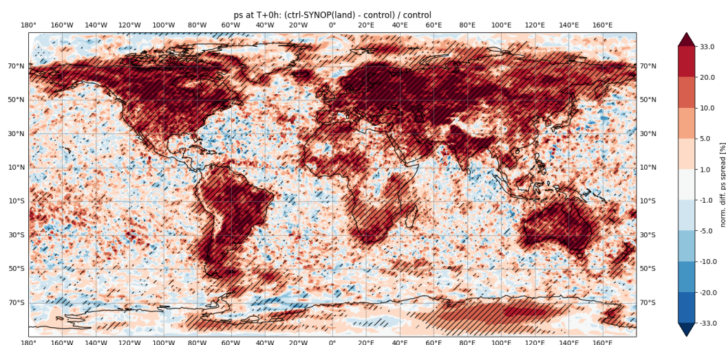
Figure 4 A spatial map of the surface pressure analysis uncertainty increases when real surface observations on land are removed from the control experiment, for June 1-30, 2023. The diagonal lines superimposed on the shading indicate regions where the change in EDA spread is statistically significant at the 95 % level.
