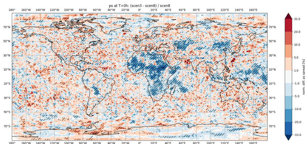
Figure 5 Upper panel: the map of surface observations used in SC 3. Lower panel: The reduction in surface pressure analysis uncertainty for SC 3 when compared with the SC 8 for June 1-30, 2025. This illustrates the impact of surface network in assimilated in SC 3 but not included in SC
