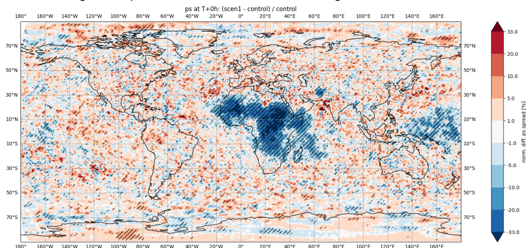
Figure 3 The percentage reduction in the surface pressure analysis uncertainty for SC 1, when compared with the control experiment for June 1-30, 2023. Negative values (blue shading) indicate the regions where the surface pressure analysis uncertainty for SC 1 is improved when compared to the control experiment. The diagonal lines superimposed on the shading indicate regions where the improvement is statistically significant at the 95 % level.
